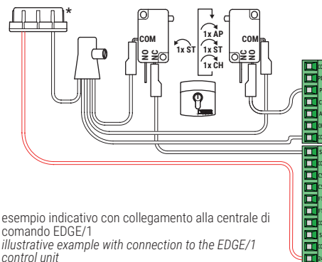
SCHEMA DI COLLEGAMENTO PASSO PASSO (AP - ST - CH) CON CONNECTION DIAGRAM STEP BY STEP (AP - ST - CH) with additional STOP contact
